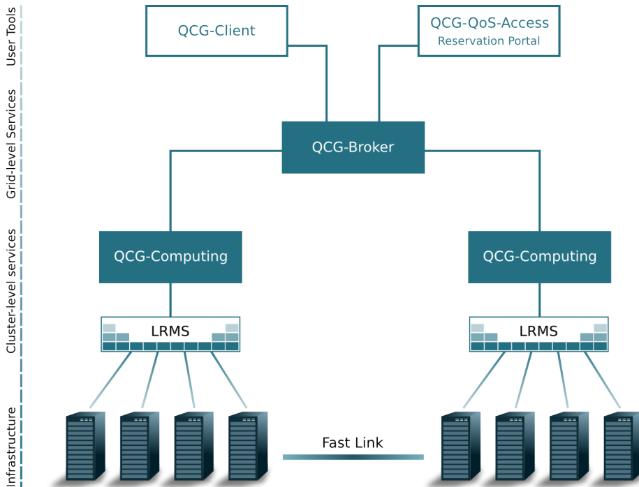
Fig. 2. The QosCosGrid middleware architecture
